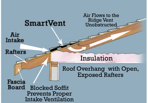
Mid-Roof Intake
