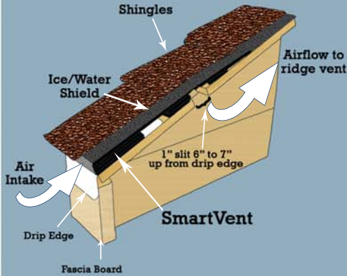
Eave Intake
